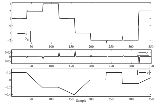
Fig. 2. Numerical example: realized closed-loop output response y and desired output response y_M (top), tracking error \varepsilon (middle), scheduling signal p (bottom).
